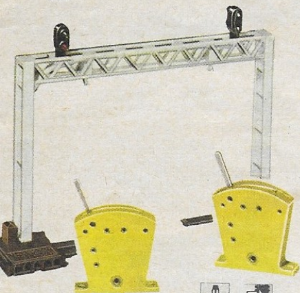
R.573 Colour Light Signal Gantry Set. Operates from 12/15 Volts A.C./D.C. Bases CLIP-FIT to Track. Includes 2 Lever Frame Sections. Can be operated by Automatic Train Control Sets.
