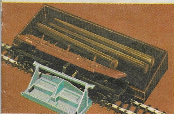
R.345 Side Tipping Flat Car. As Car passes Collection Bin the carrying frame automatically tilts and logs roll off into bin. Operating Ramp CLIP-FITS to Track.
