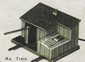
RT.267 Fog Signal. As Train passes hut a 'maroon' is automatically fired. Mechanically operated. Caps not included.
