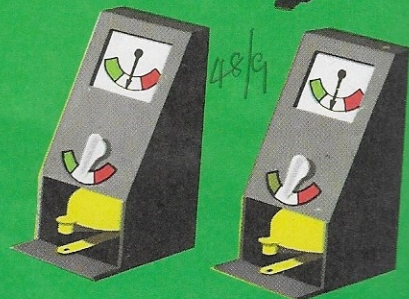
R.263R POINT OPERATED SIGNAL—Right Hand. Clip Fits to point and the action of switching the point automatically changes the signal.
