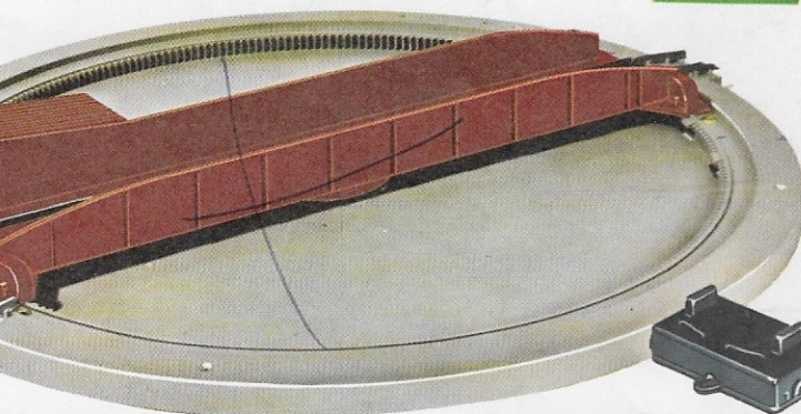
R.408 ELECTRICALLY OPERATED TURNTABLE. Control switch. 12 volts DC. Enables locomotives to be turned round or directed into any one of the three track outlets
