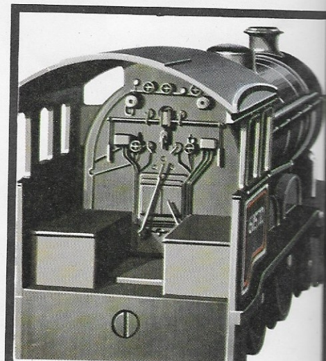
View showing cab interior detail of B.12 Locomotive.
